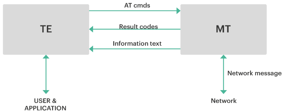
Figure 1 AT command interface
